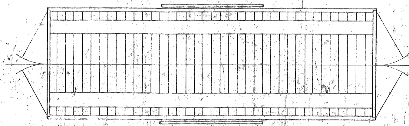
C.L.C. FOUR-WHEELED COVERED CARRIAGE TRUCK.
